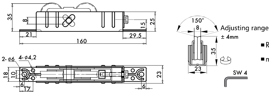
ALU CS 120kg H27 bogie wheel
