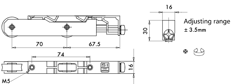
ALU CS 150kg bogie wheel
