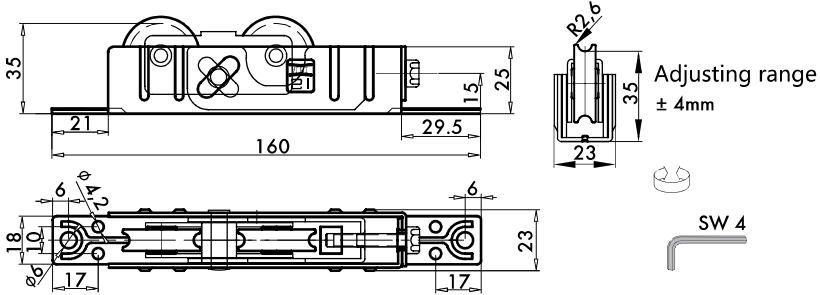
ALU CS 120kg H35 bogie wheel
